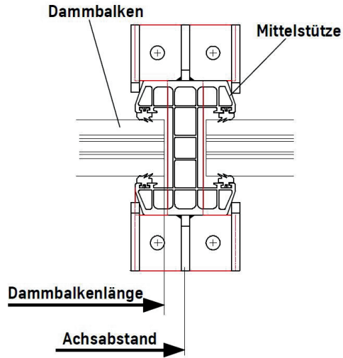
Detail A
