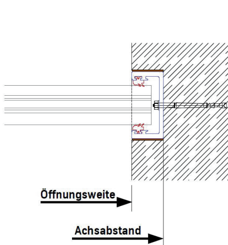
Detail C
