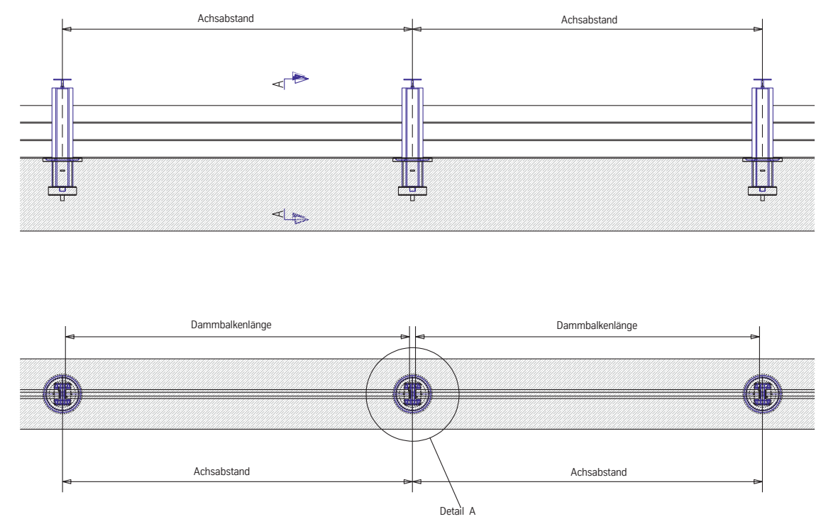
Detail A
